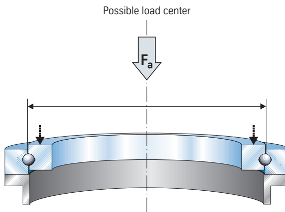
Figure 35: Loading principle of the axial reduction measurement
