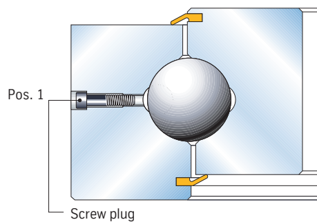
Figure 42: Single-row ball bearing with grease sampling port
