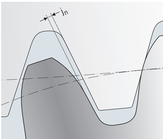
Figure 20: Backlash
