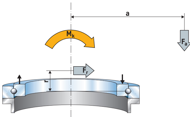
Figure 12: Axial load "application from above"
