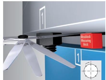
Figure 37: Basic setup for measuring the axial reduction with a feeler gauge
