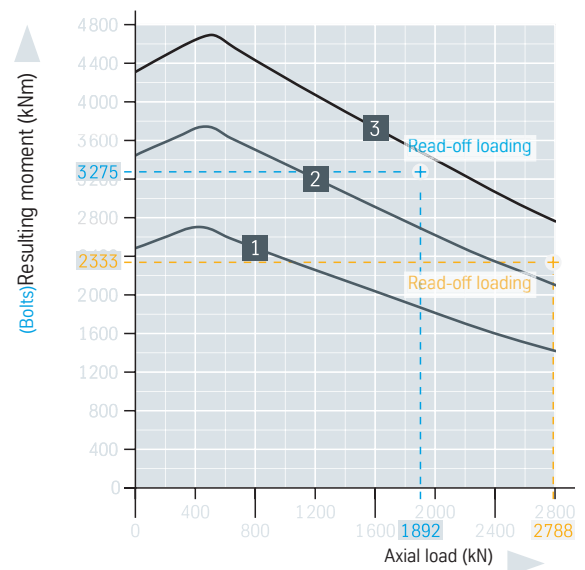
Utilization period curves · 30 000 revolutions
