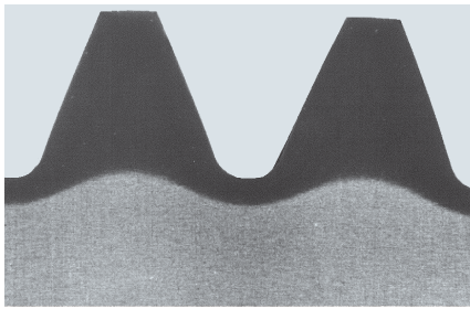
Figure 18: Circulation hardening
