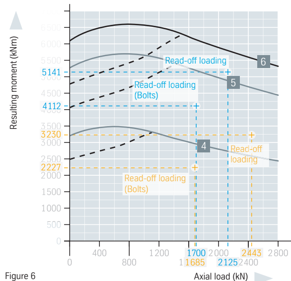
Static boundary load curves
