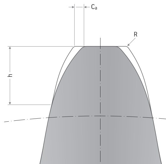
Figure 23: Tip flank profile
