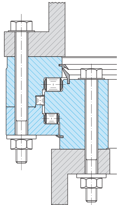
Figure 25: Companion structure
