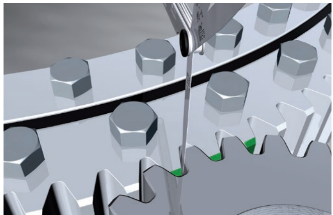
Figure 30: Backlash measurement
