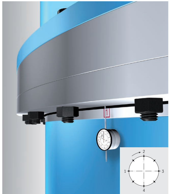
Figure 34: Basic setup for measuring the tilting clearance
